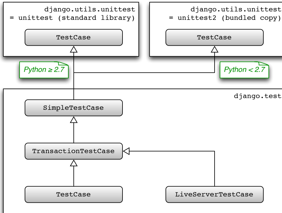
Fig. 3.1: Hierarchy of Django unit testing classes
